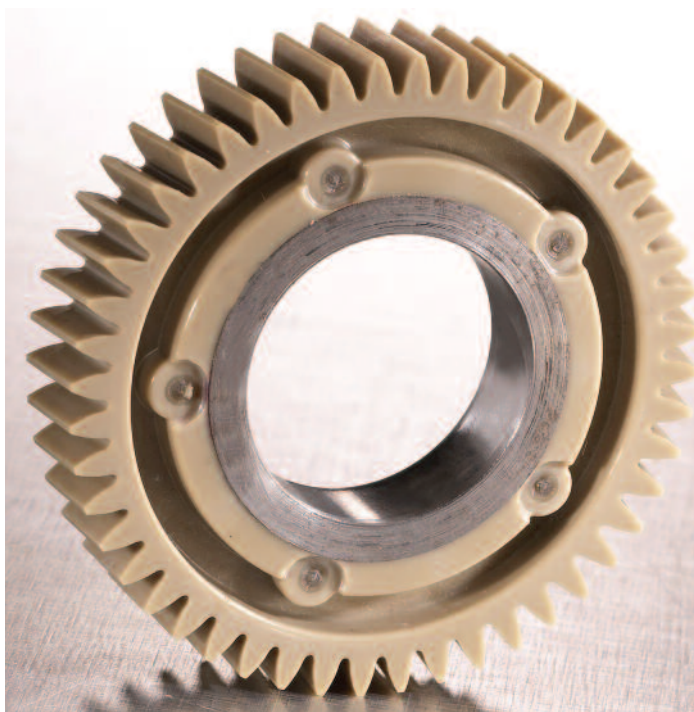
VICTREX® PEEK polymer replaces iron in design of gears used in balance shaft modules to deliver durability, reliability and improve efficiency.
